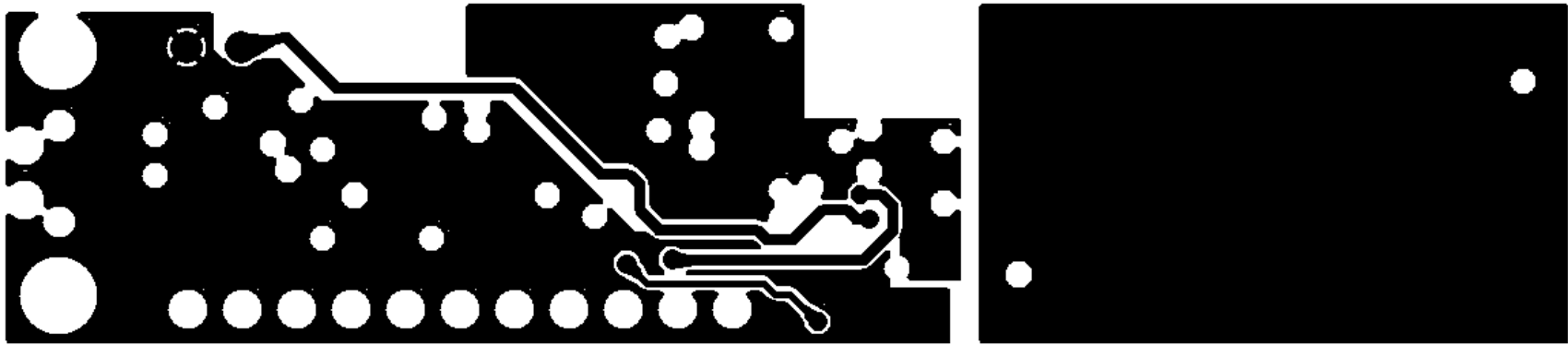
Figure 14: 3rd layer layout
