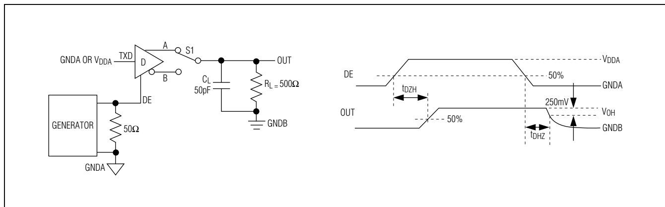
Figure 4. Driver Enable and Disable Times ( t_{DHL} , t_{DZH} )
