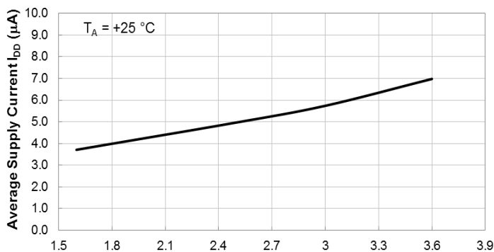
Average Supply Current vs Supply Voltage
