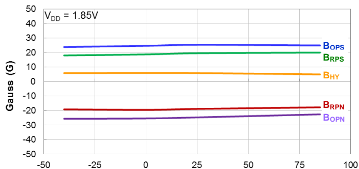
Switch Points B_{OP} and B_{RP} vs. Temperature
