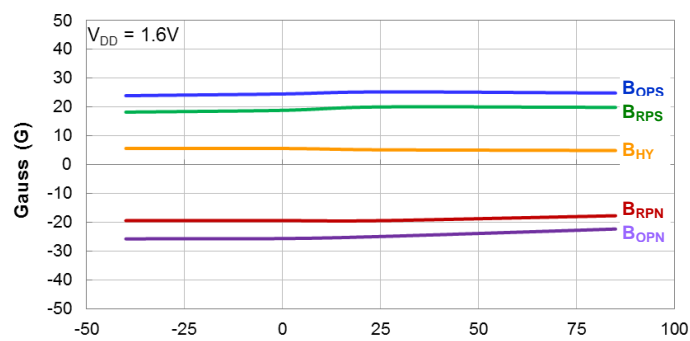
Switch Points B_{OP} and B_{RP} vs. Temperature
