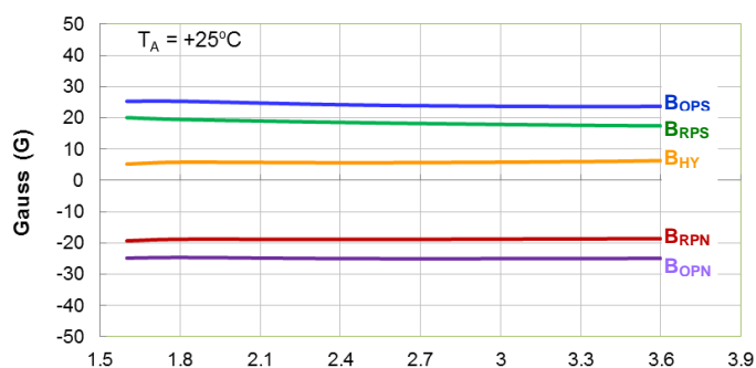
Switch Points B_{OP} and B_{RP} vs. Supply Voltage
