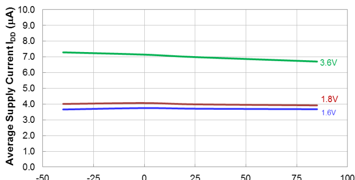
Average Supply Current vs Temperature
