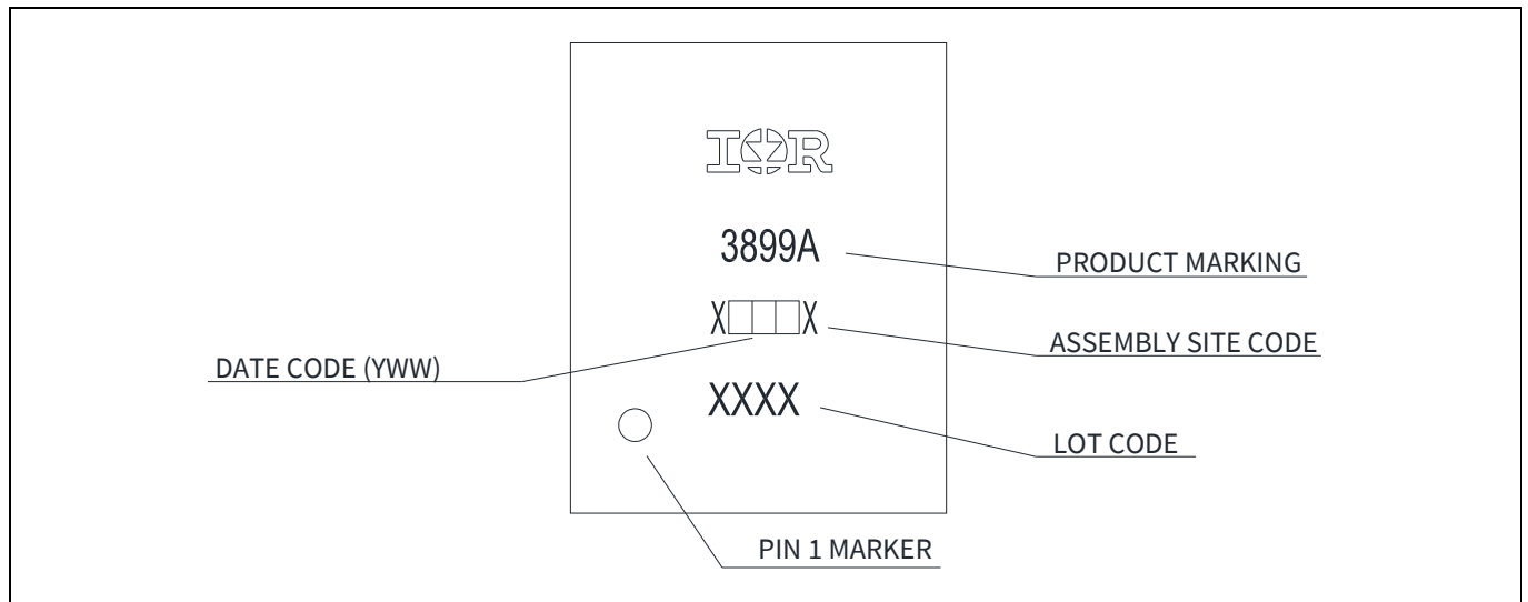
Figure 22 Package Marking
