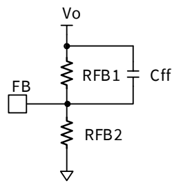
Figure 12 Configuration of feedforward capacitor, Cff.
